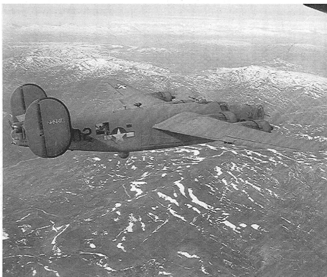
A typical "Mickey Ship" note the radome hung in the place of the ball turret.
